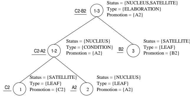
Figure 7.6: Example of a valid text plan for the problem in (7.3)–(7.4).
